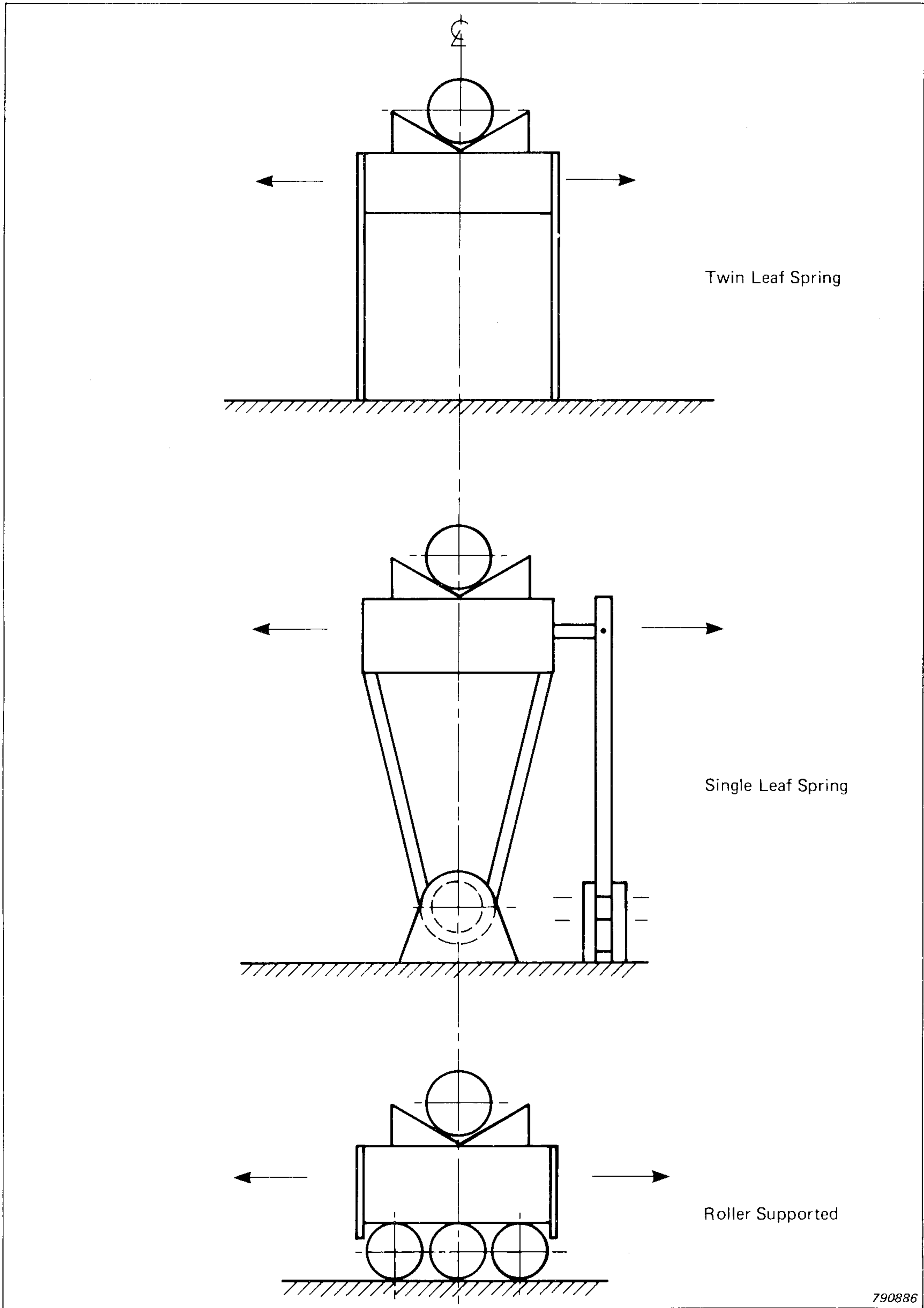
Fig.11. Examples of soft suspension types
