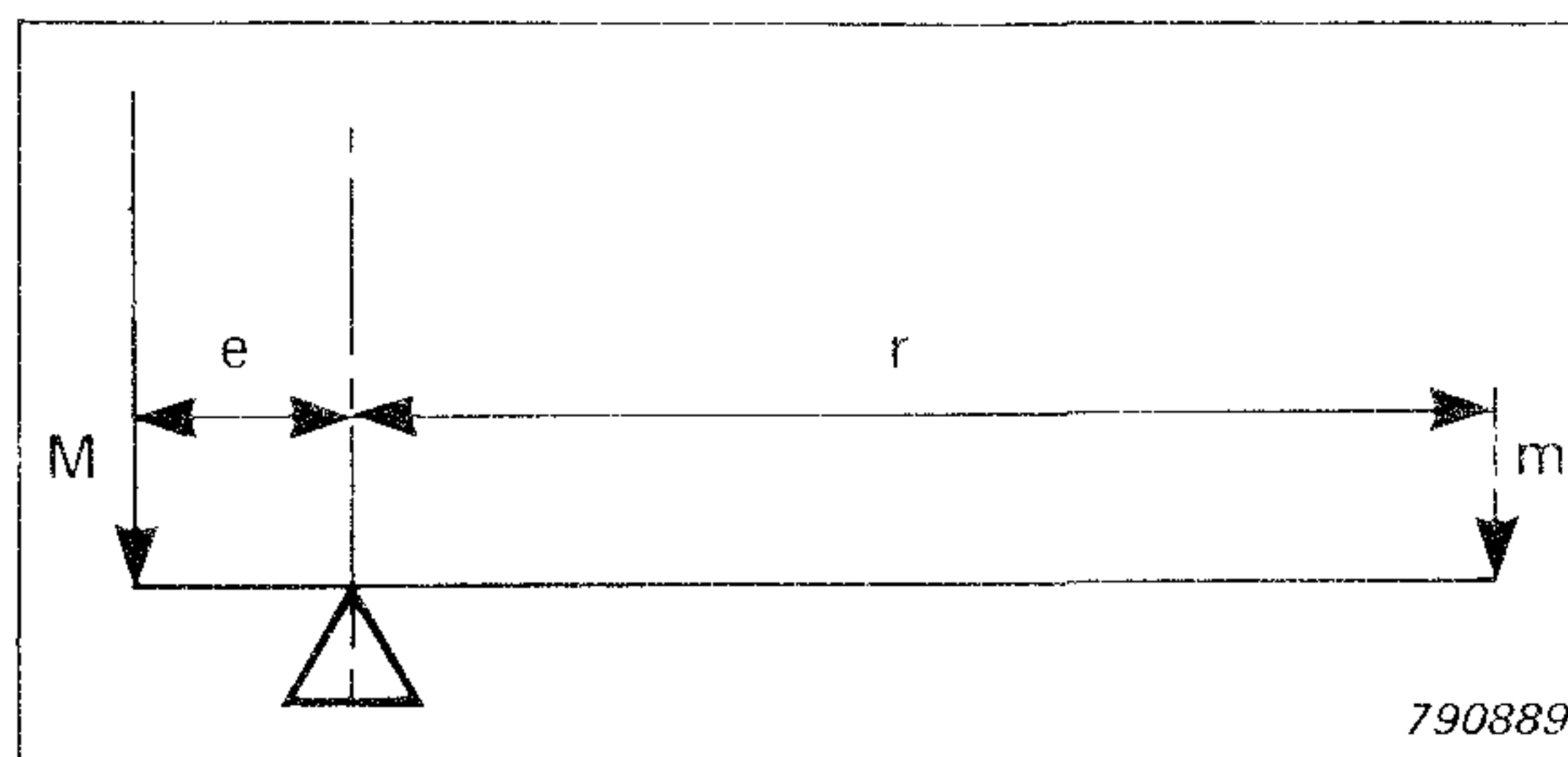
Fig.2. Displacement of Centre of Mass
