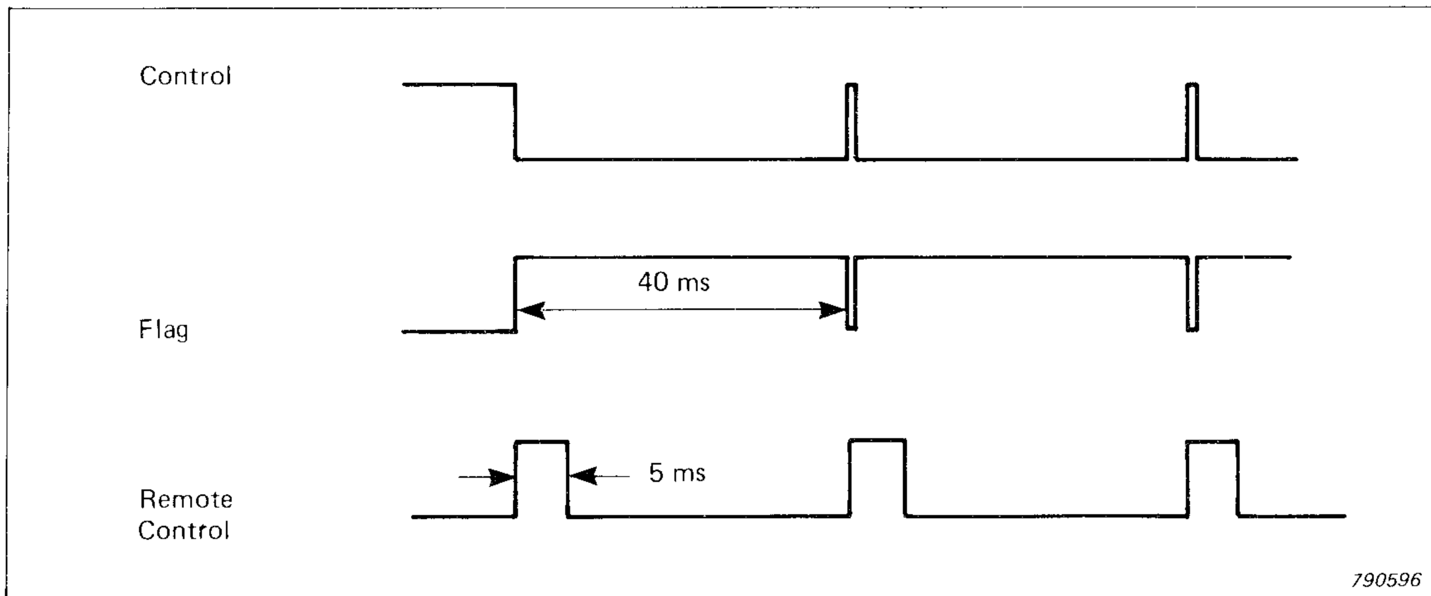
Fig.2. Timing diagram of the Interface
