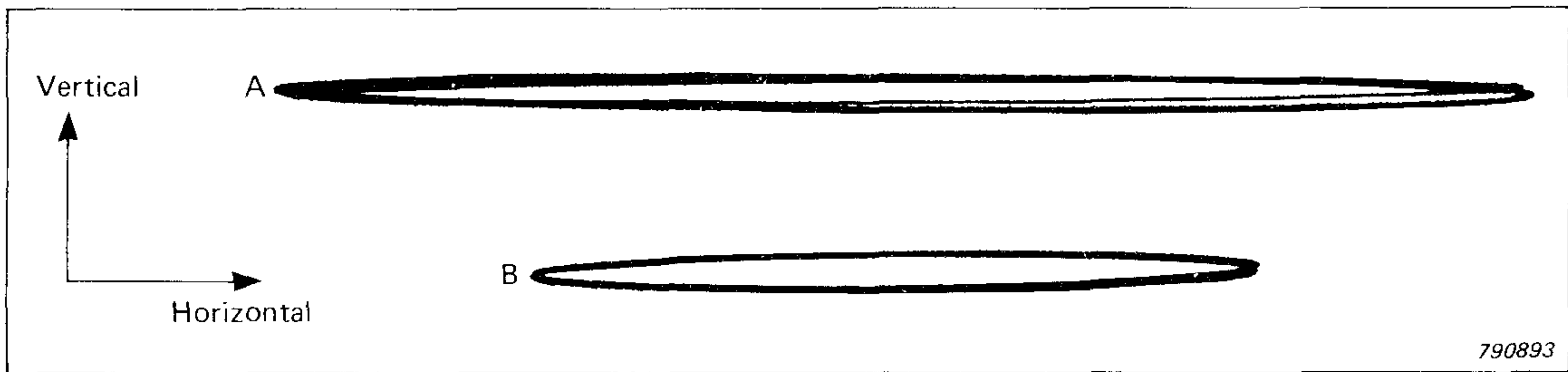
Fig.12. Vibration at support A and B on a balancing machine (Type 3905 at 3000 r.p.m.)
