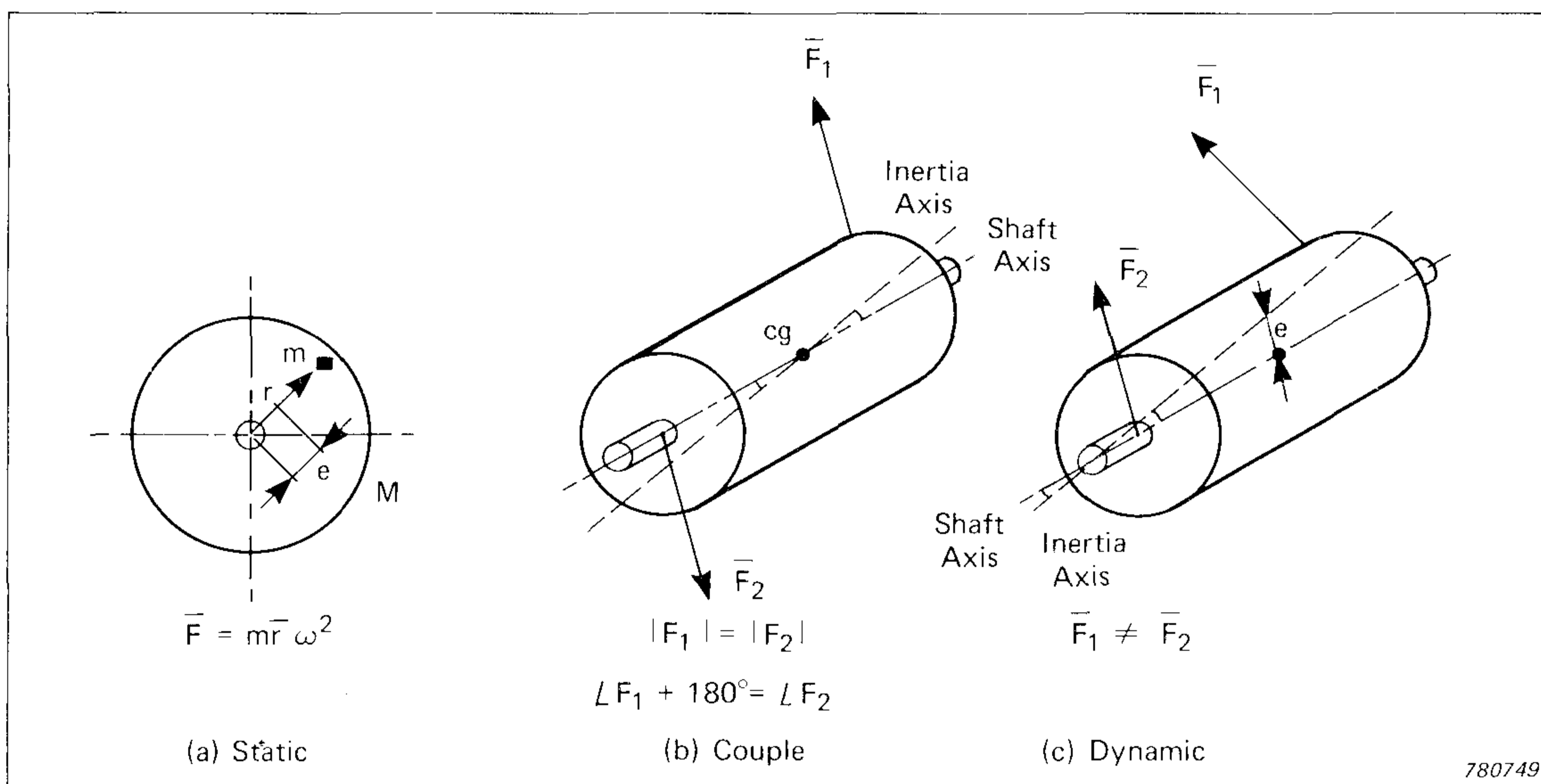
Fig.1. Rigid Rotor Unbalance
