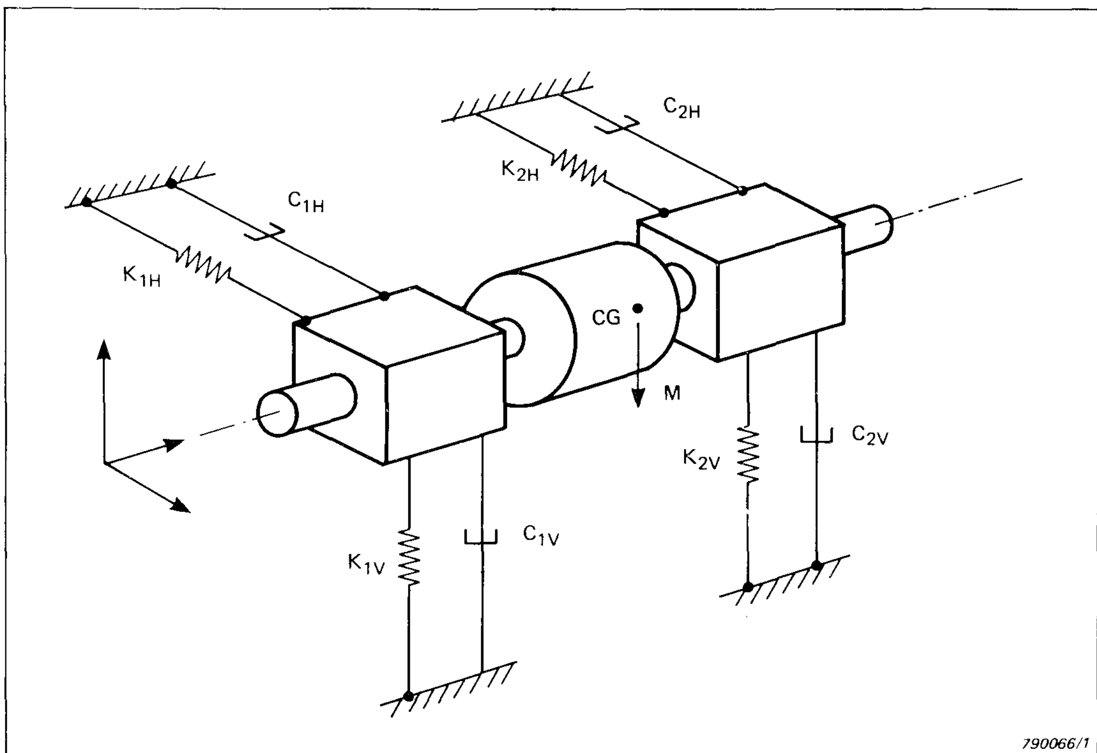
Fig.13. Linear Model of complete machine
