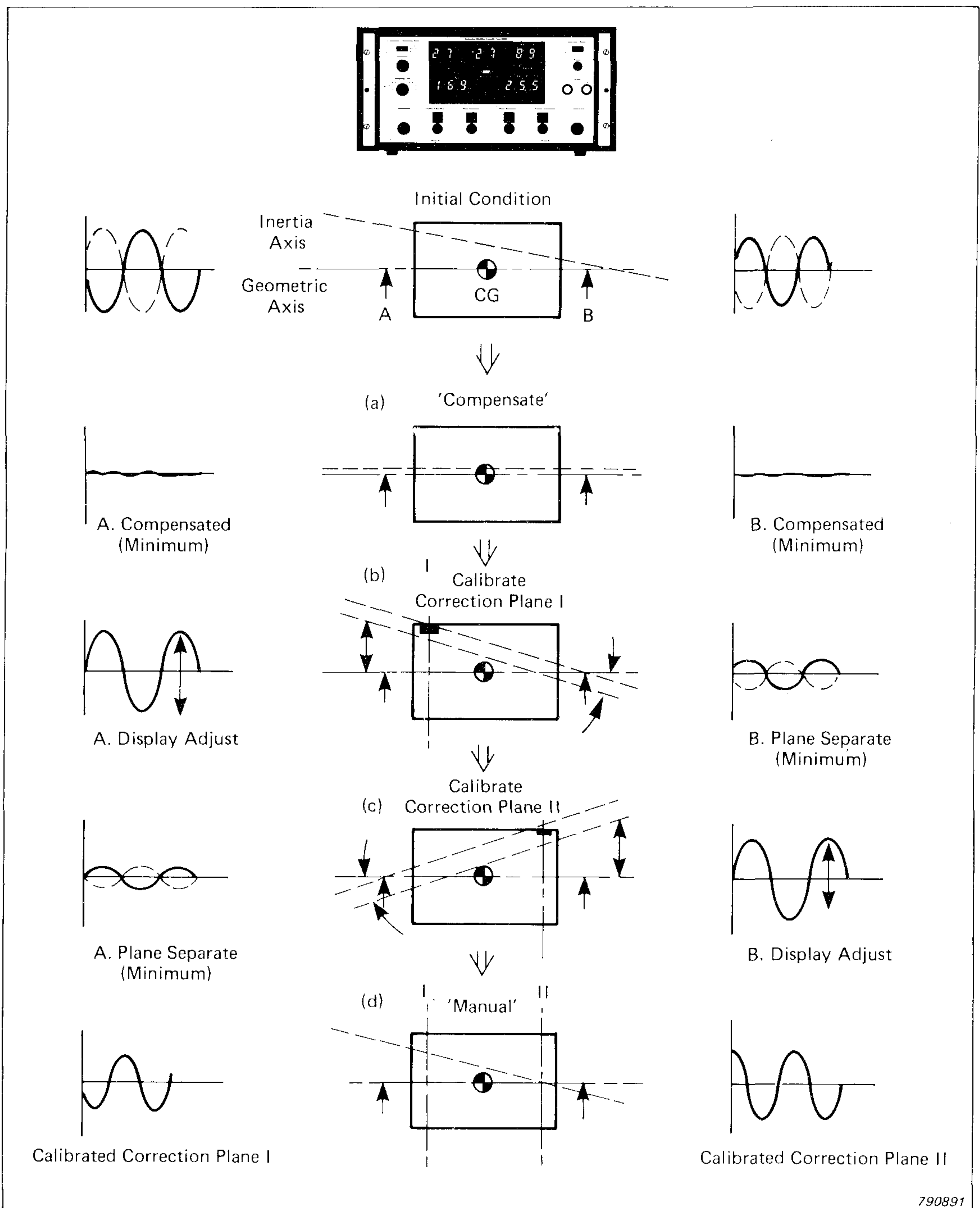
Fig.3. Calibration Procedure
