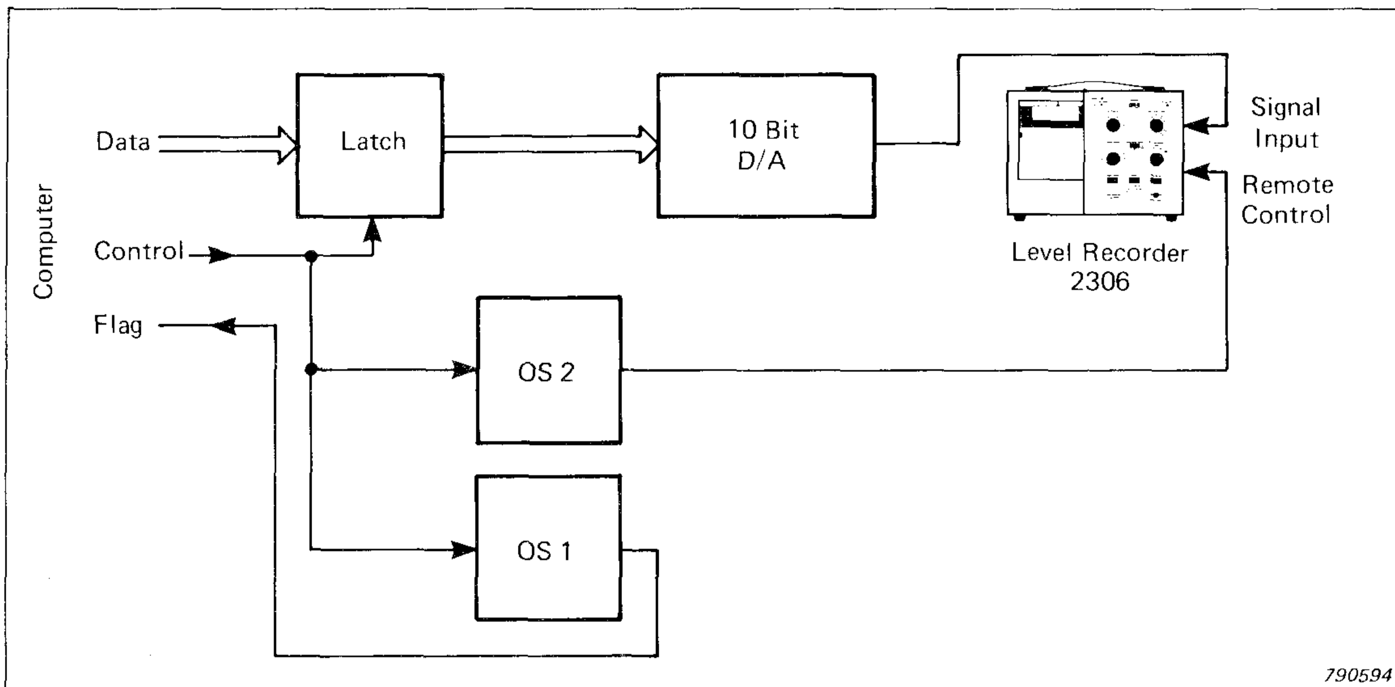
Fig. 1. Block diagram of the Interface
