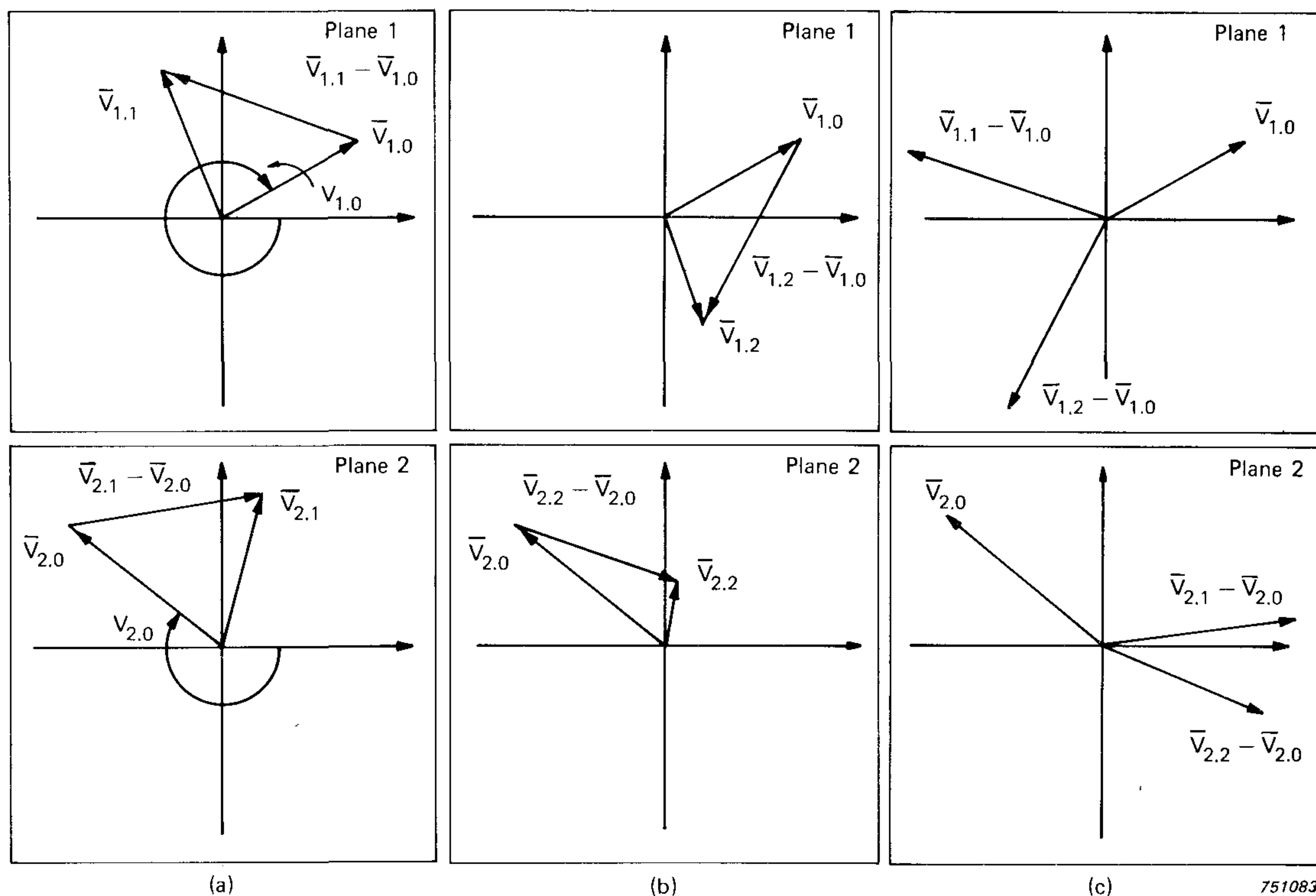
Fig. 6. Vectorial representation of the vibration levels
