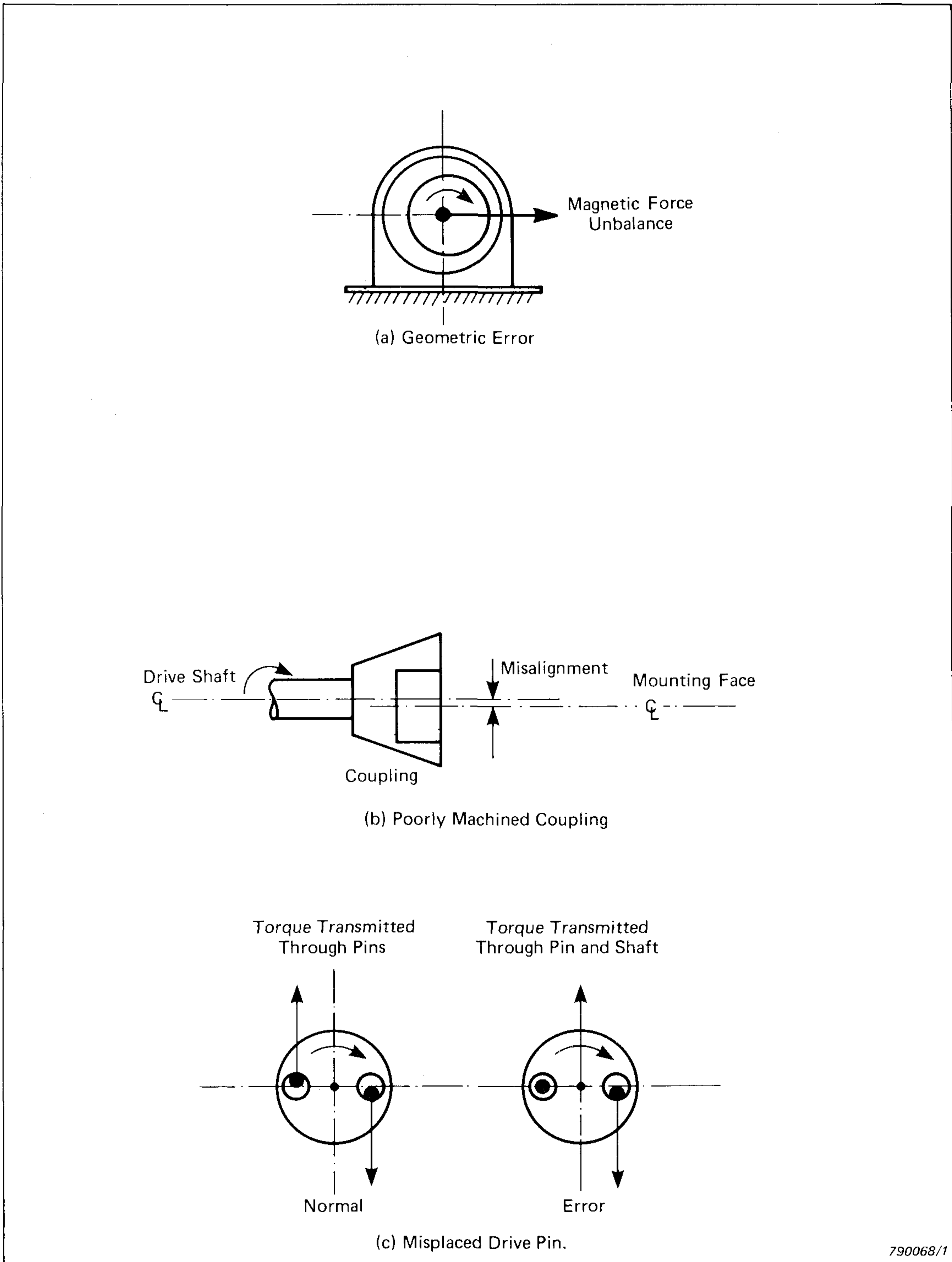
Fig.15. Same quasi-unbalance sources
