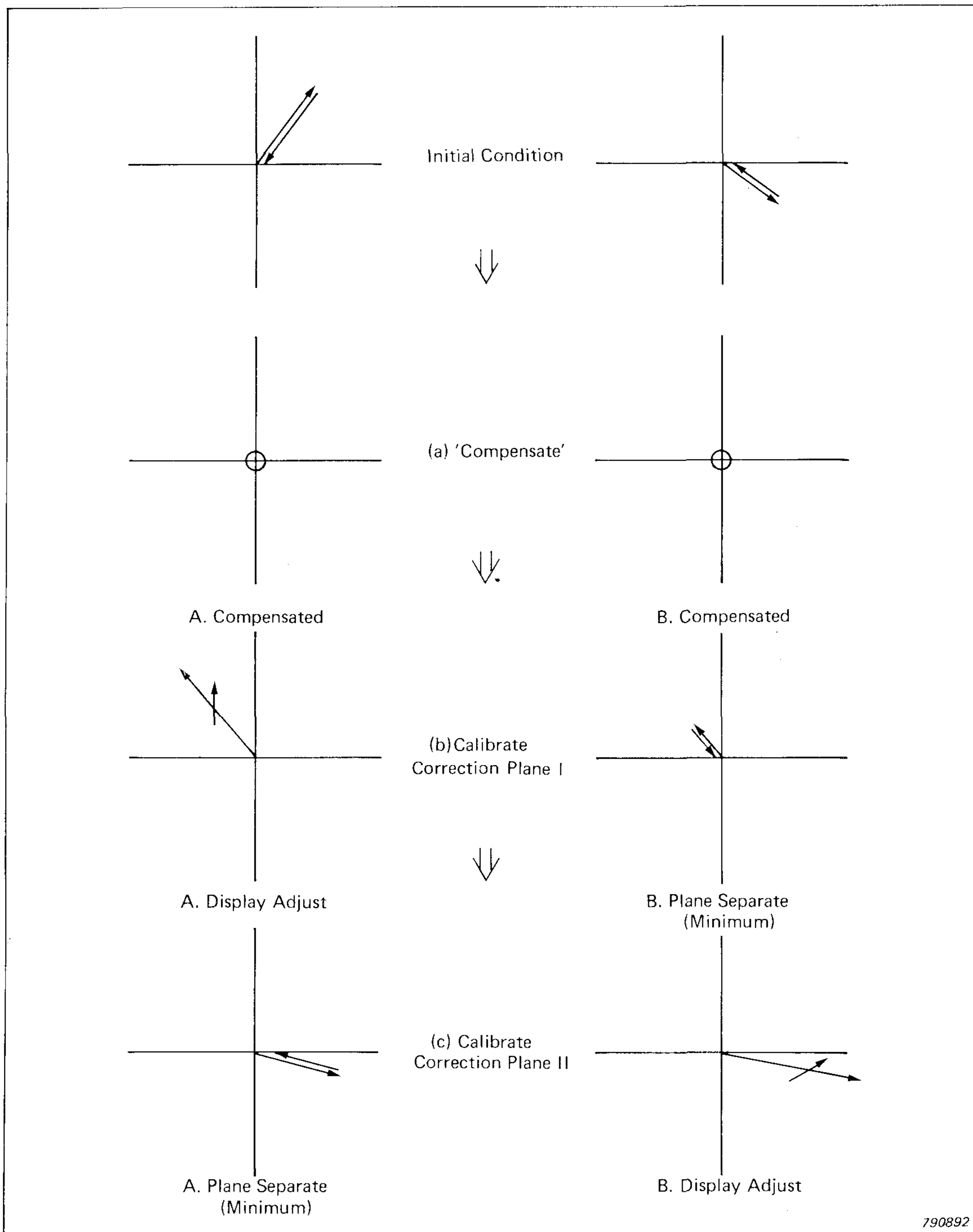
Fig.4. Calibration Procedure — Vector Format
