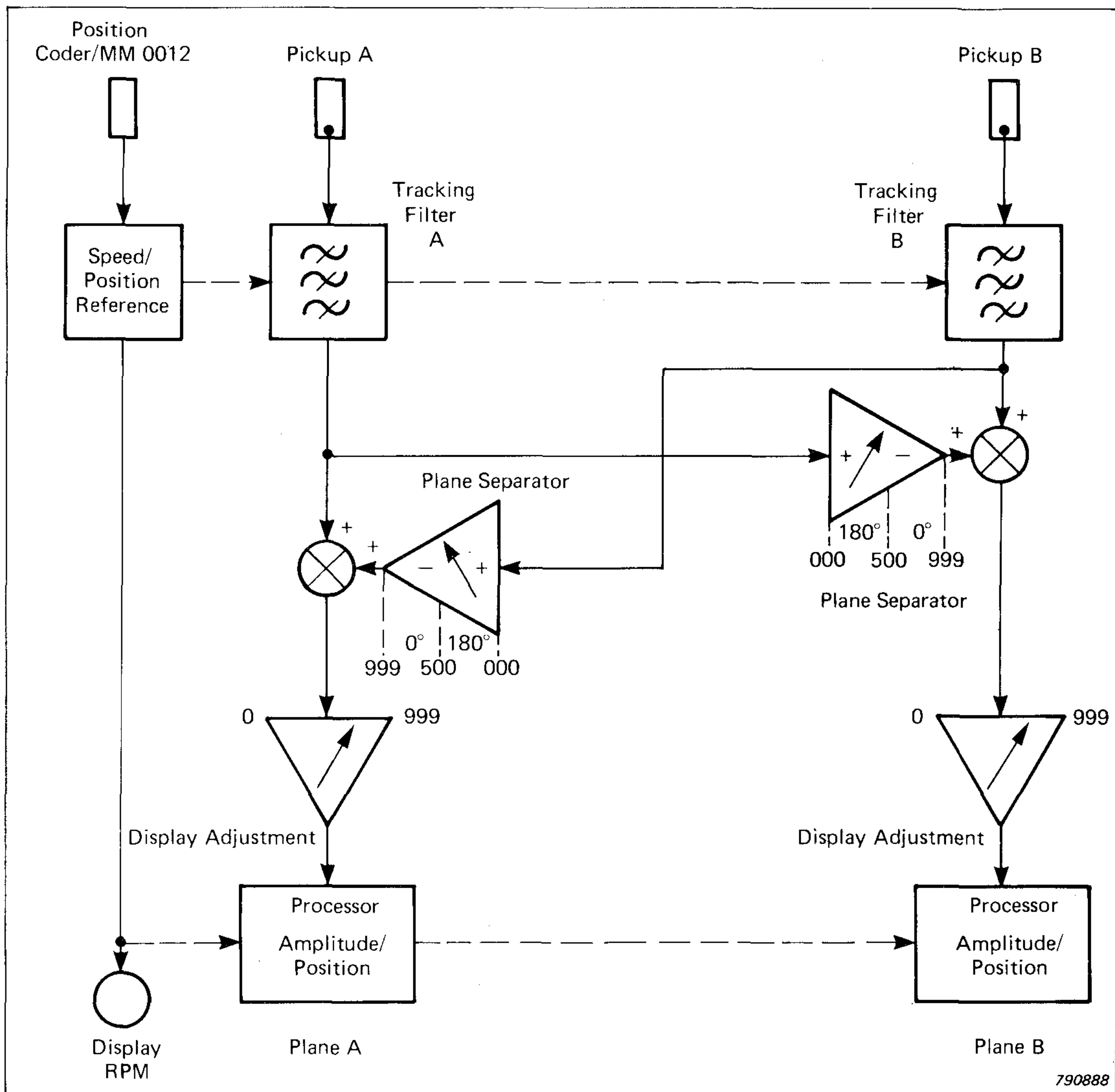
Fig.10. Functional Diagram of 2504 system
