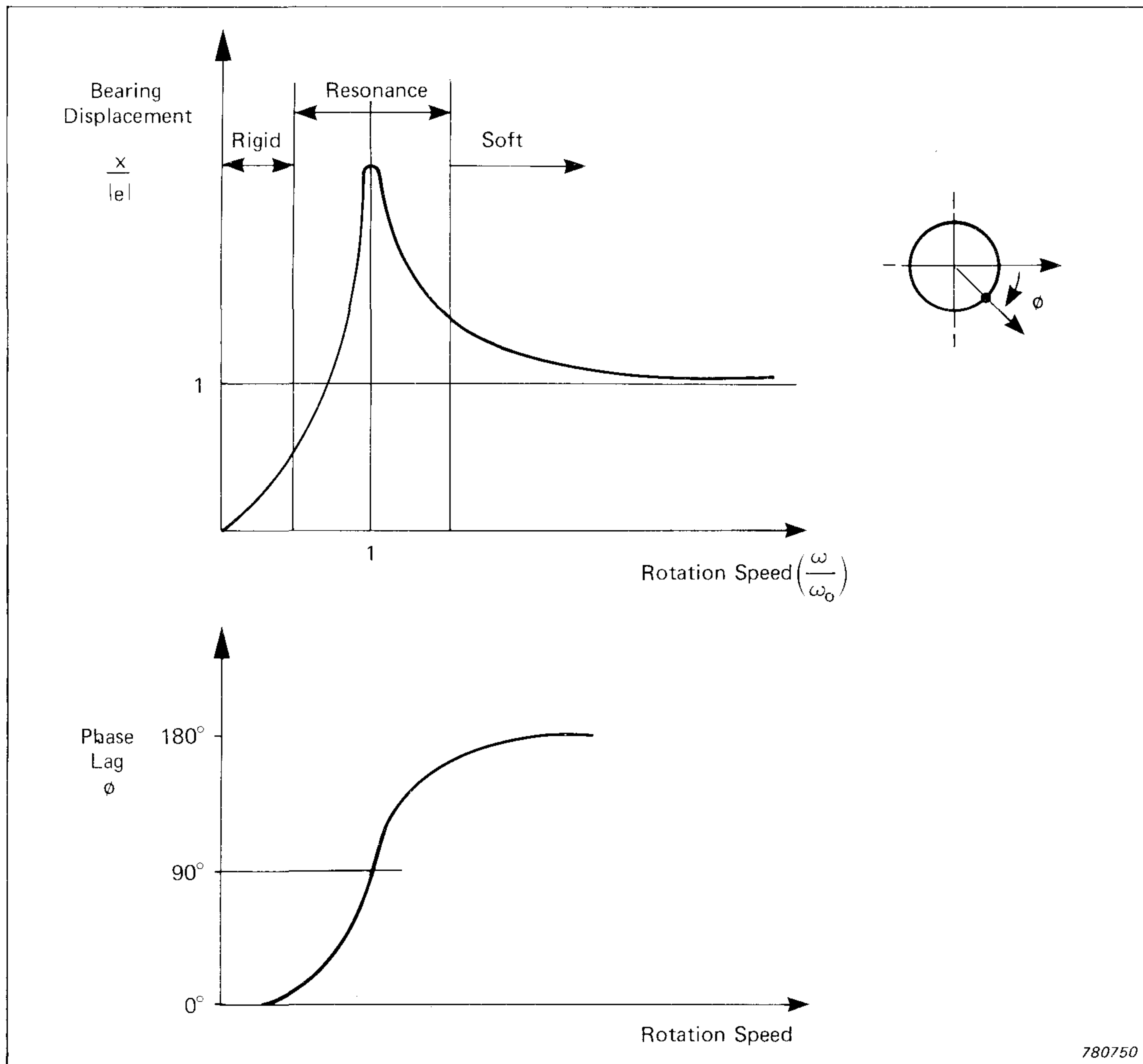
Fig.5. Response of a single degree of freedom support system to unbalance force input
